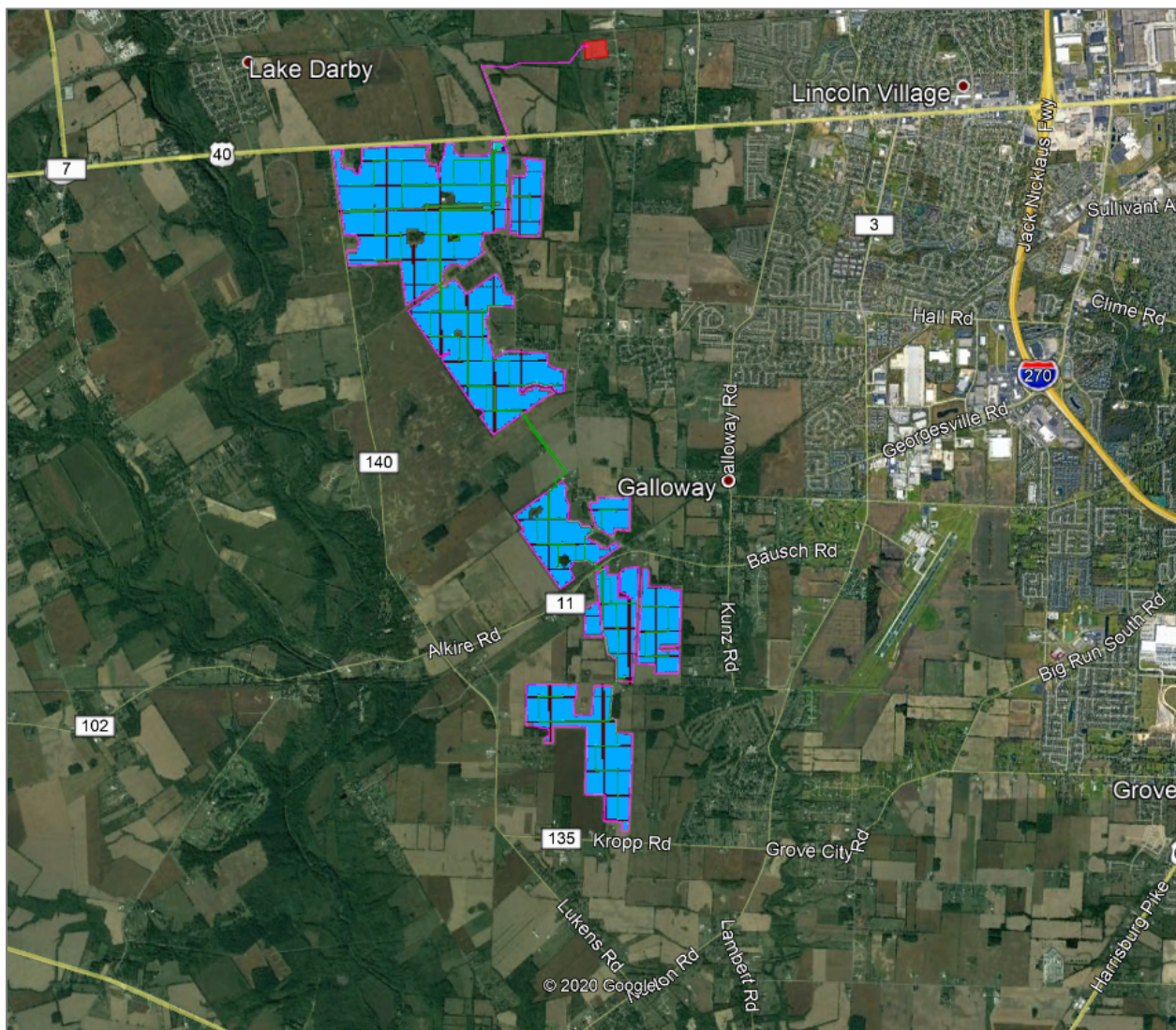
Figure 1 Project Layout
