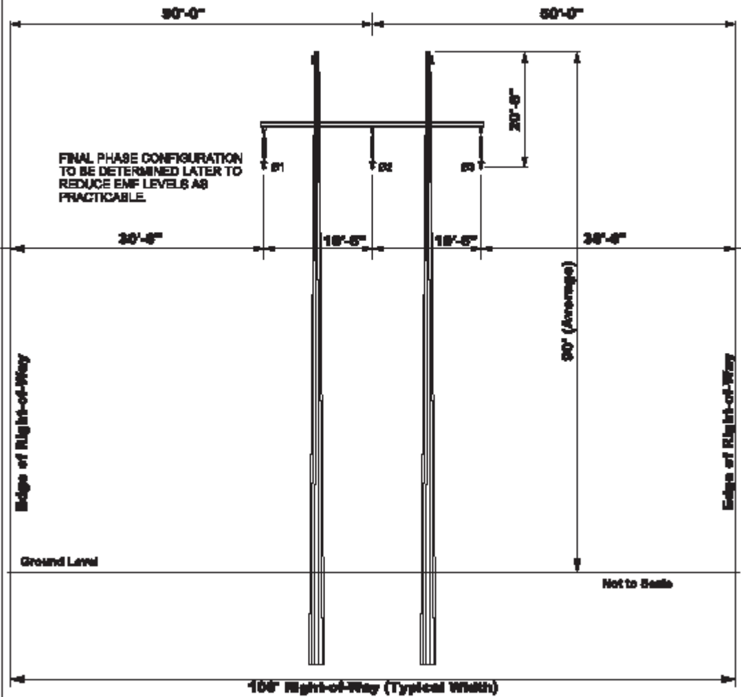
TYPICAL RIGHT-OF-WAY CROSS SECTION
