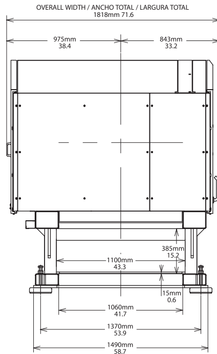
Clamp End View
