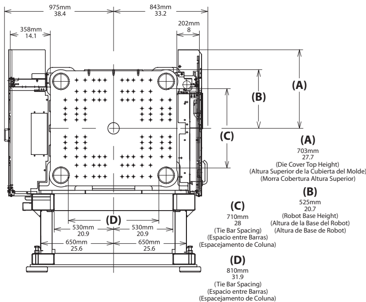
Stationary Platen
