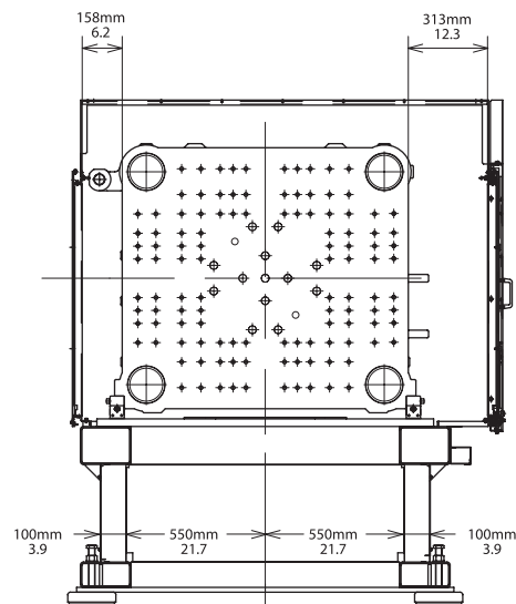
Stationary Platen
