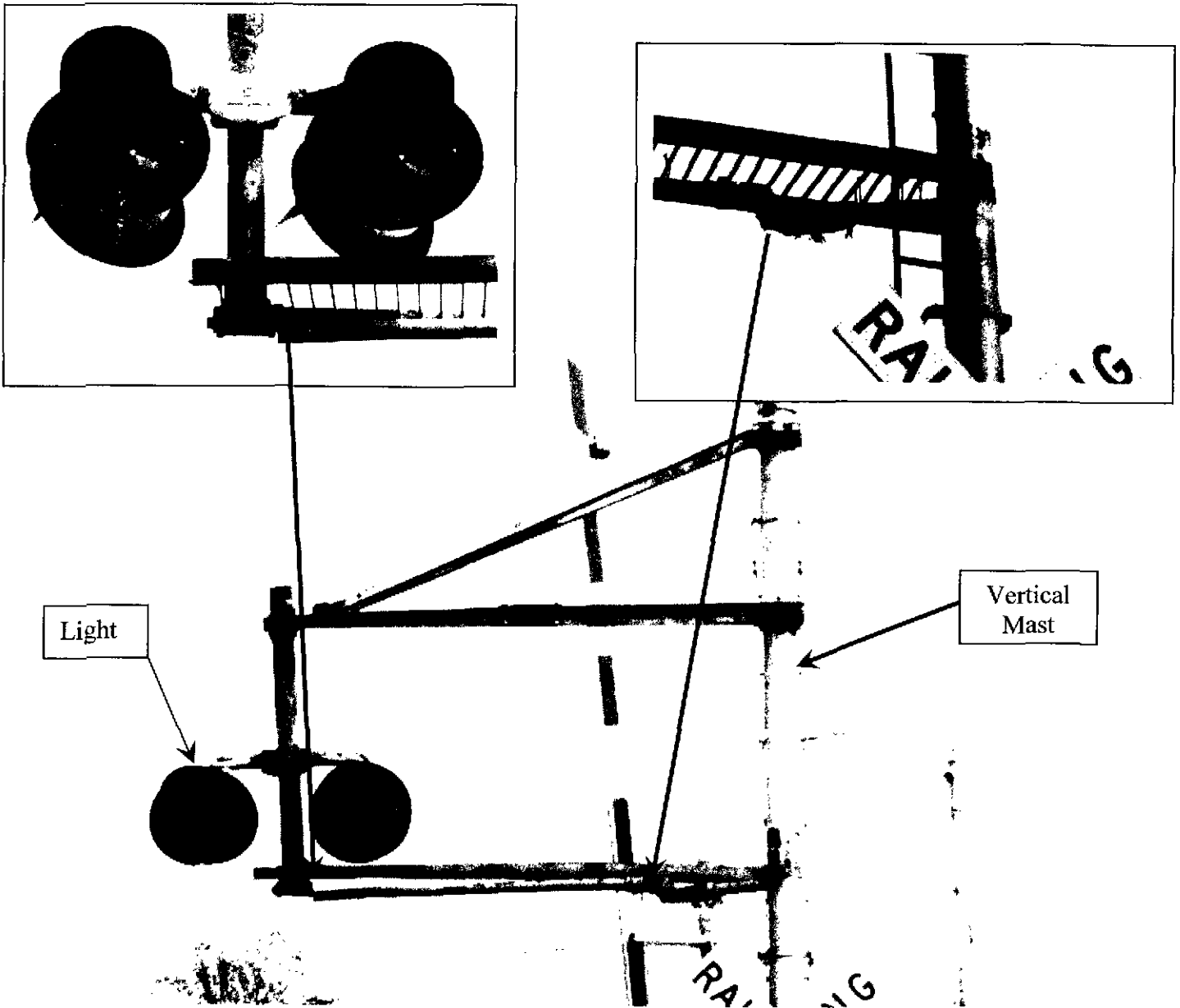
Photograph of Damaged Cantilever State Street Crossing – (473-711A)
