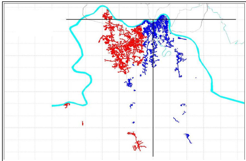
Figure 3-4: The extent of propane flow into the northern Kentucky part of the system from the Kentucky propane-air peaking plant at peak demand flow.
