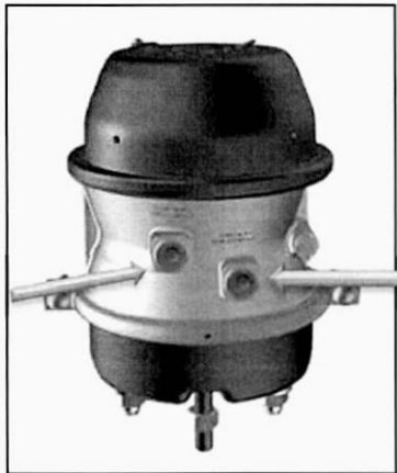
Square-shaped air fitting ports
