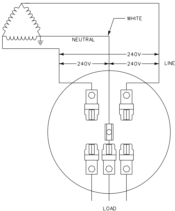
3 WIRE 240 VOLT THREE PHASE SELF CONTAINED CENTER PHASE DISCONNECT
