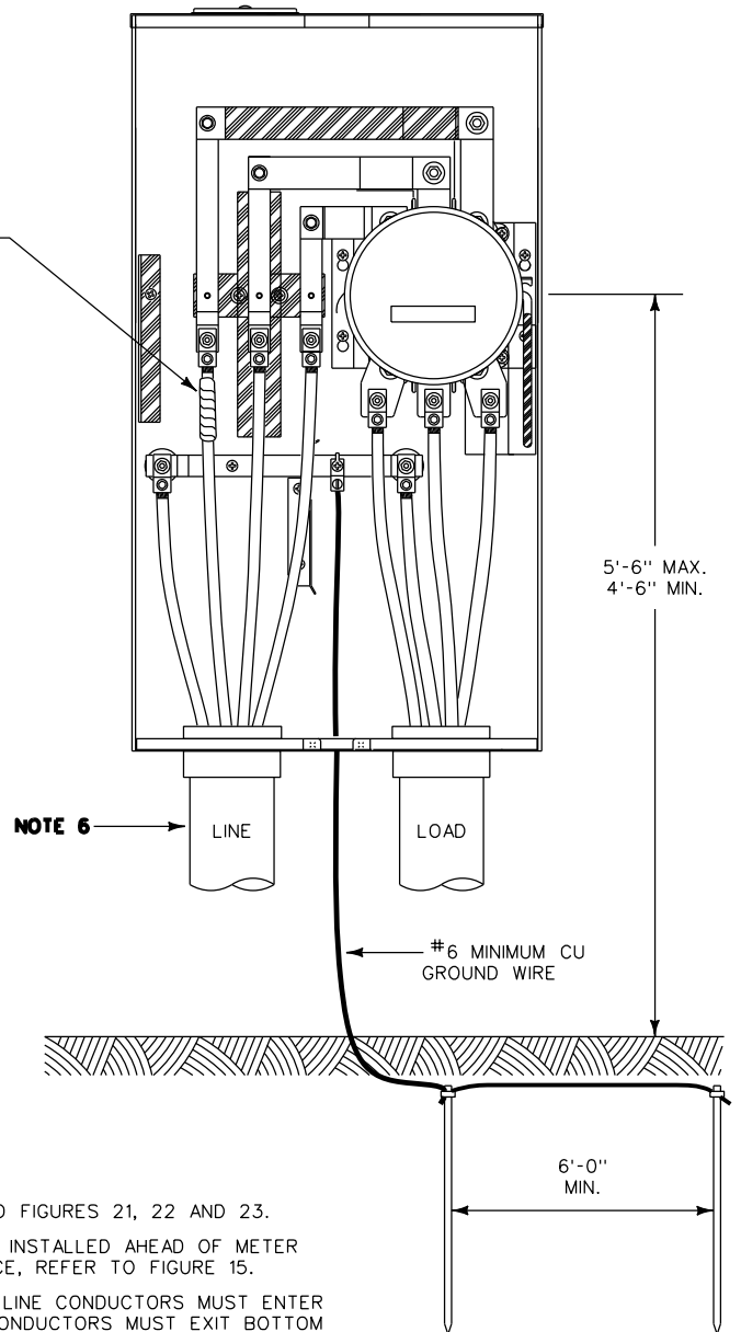
THREE PHASE 4 WIRE 320 AMP SOCKET METER BOX WITH BY-PASS SWITCH NOTES 1 AND 2
