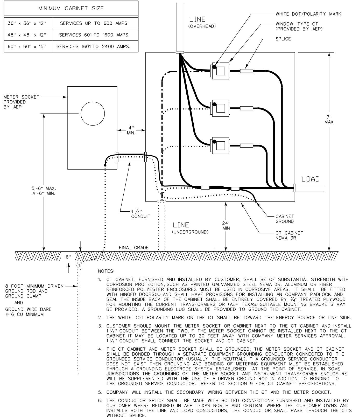
CURRENT TRANSFORMER CABINETS OVERHEAD OR UNDERGROUND SERVICE WINDOW TYPE CT'S FIGURE 10
