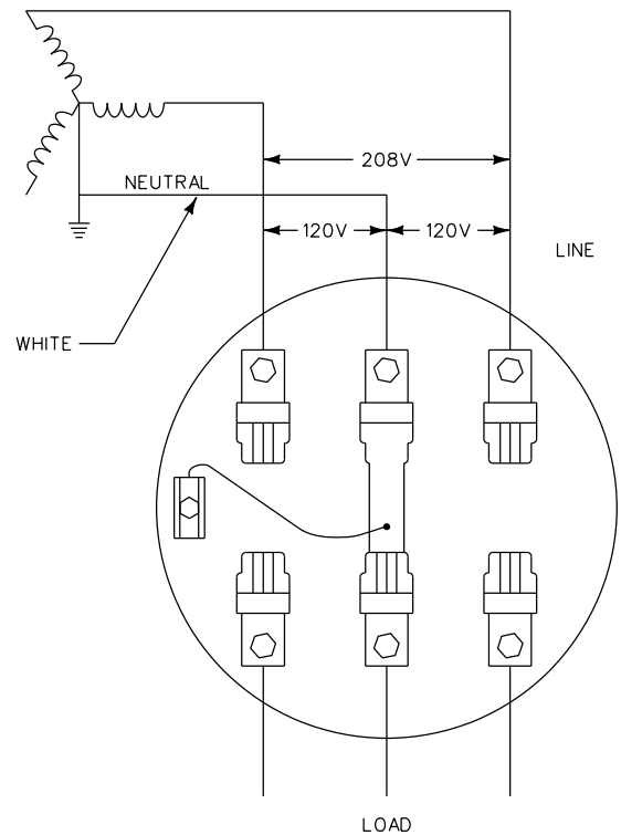
3 WIRE NETWORK 120/208 VOLT SINGLE PHASE SELF CONTAINED
