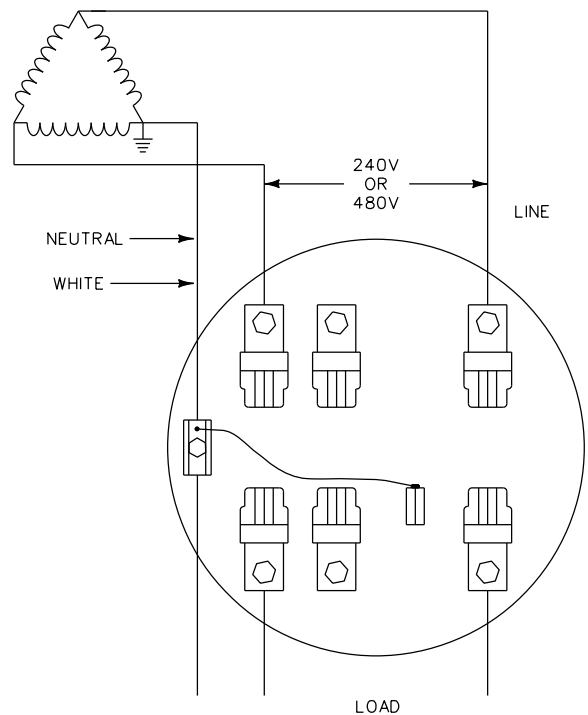
3 WIRE 240 OR 480 VOLT THREE PHASE SELF CONTAINED 7 TERMINAL SOCKET
