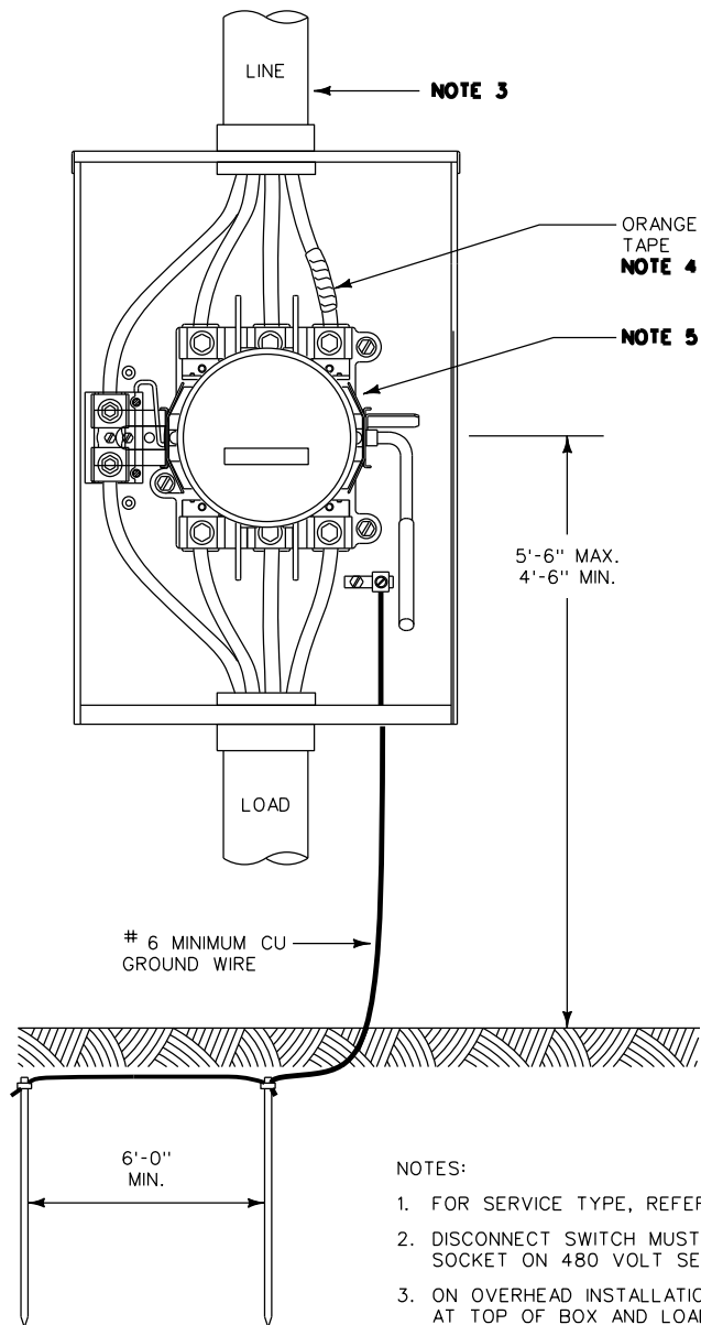
THREE PHASE 4 WIRE 200 AMP SOCKET METER BOX WITH BY-PASS SWITCH NOTES 1 AND 2
