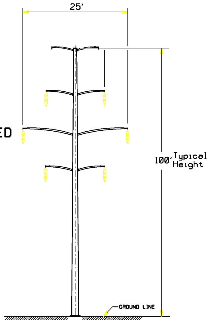
TIDD - GABLE 138kV LINE TYPICAL STRUCTURE CONFIGURATION
