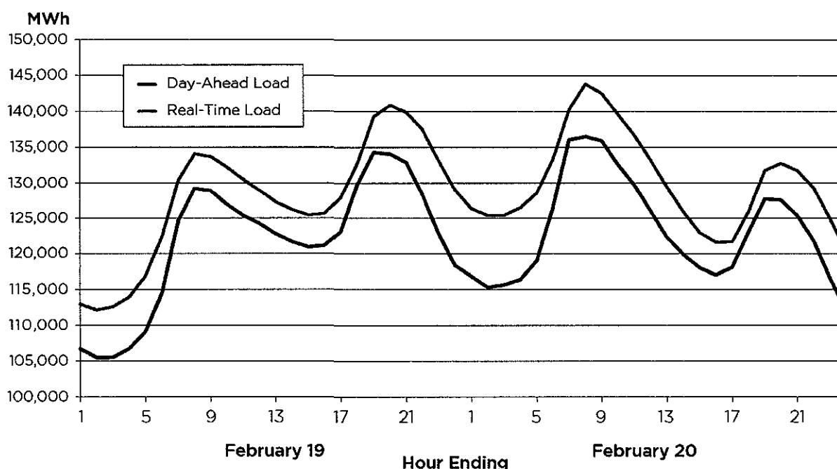
Figure 33. Day-Ahead versus Real-Time Megawatts Feb. 19 and 20, 2015
