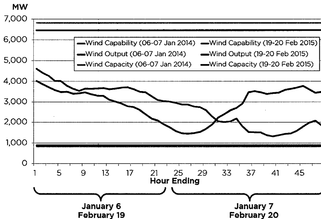
Figure 14. Wind Generation Performance at Peaks (2014 Vs 2015)
