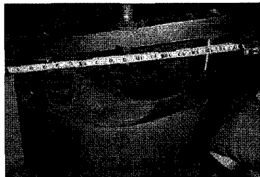
The hole in the Davis-Besse reactor head, 2002
