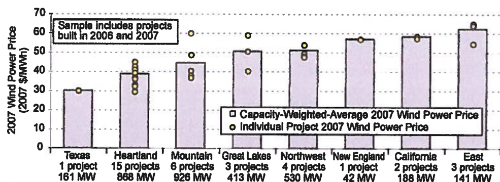
Figure 15. 2007 Wind Power Prices by Region: 2006-2007 Projects Only
