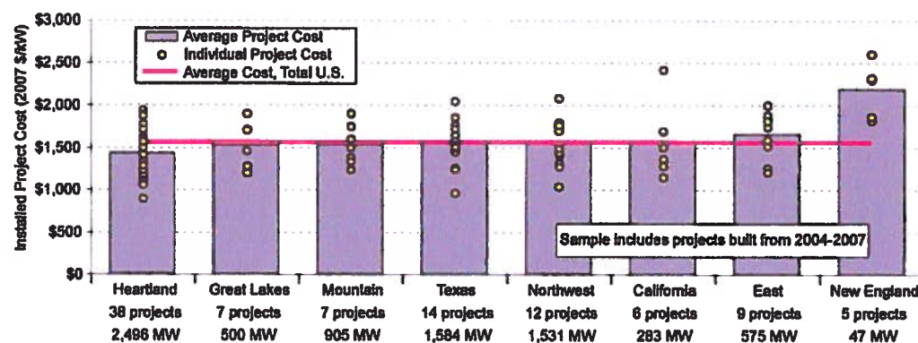
Figure 24. Installed Wind Project Costs by Region: 2004-2007 Projects
