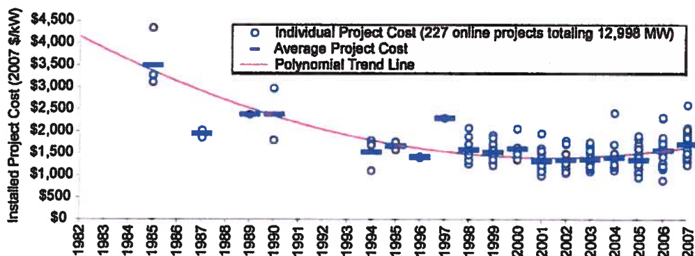
Figure 22. Installed Wind Project Costs Over Time
