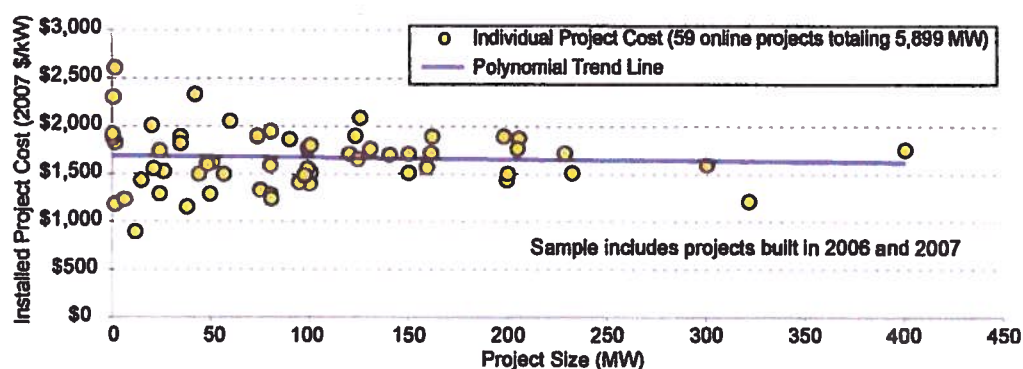
Figure 23. Installed Wind Project Costs as a Function of Project Size: 2006-2007 Projects
