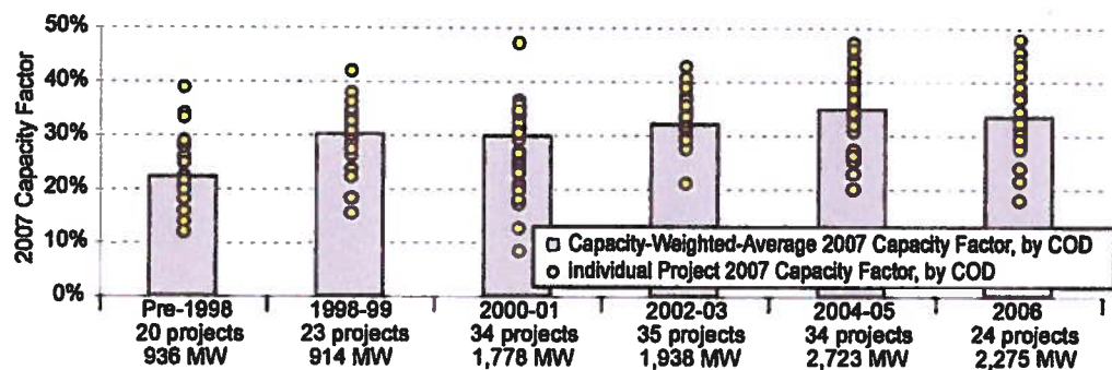
Figure 26. 2007 Project Capacity Factors by Commercial Operation Date
