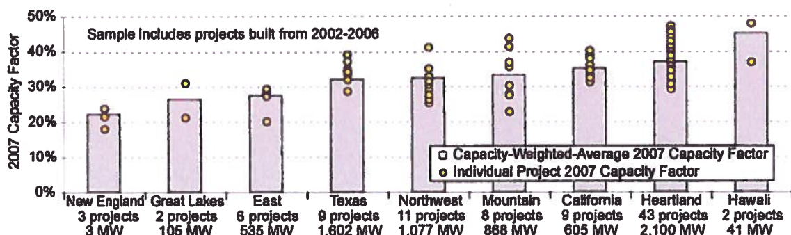
Figure 27. 2007 Project Capacity Factors by Region: 2002-2006 Projects Only
