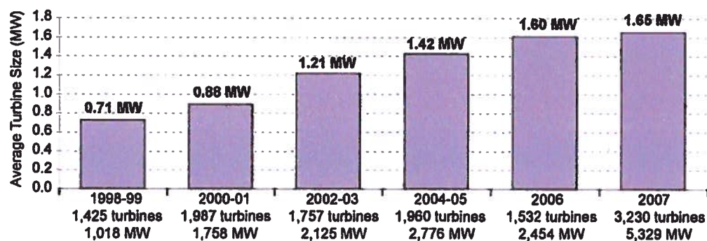
Figure 9. Average Turbine Size Installed During Period
