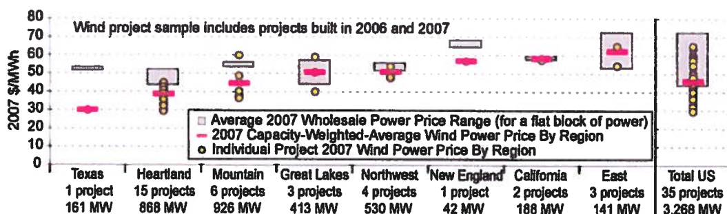
Figure 19. Wind and Wholesale Power Prices by Region: 2006-2007 Projects Only
