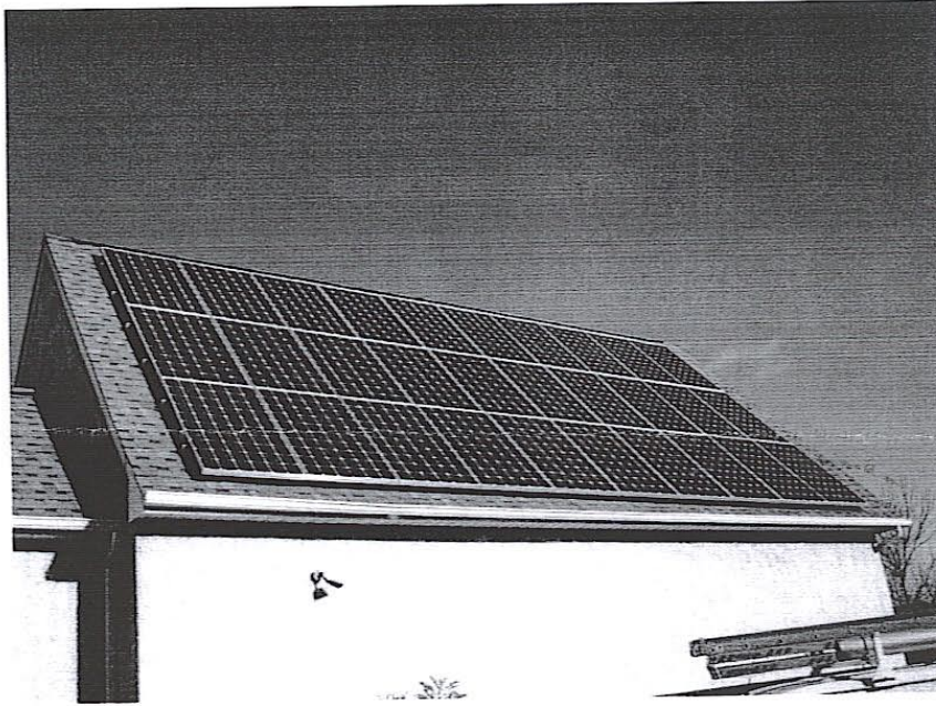
SOLAR PV ARRAY (30 SHARP 235Watt Modules, Roof-mounted)
